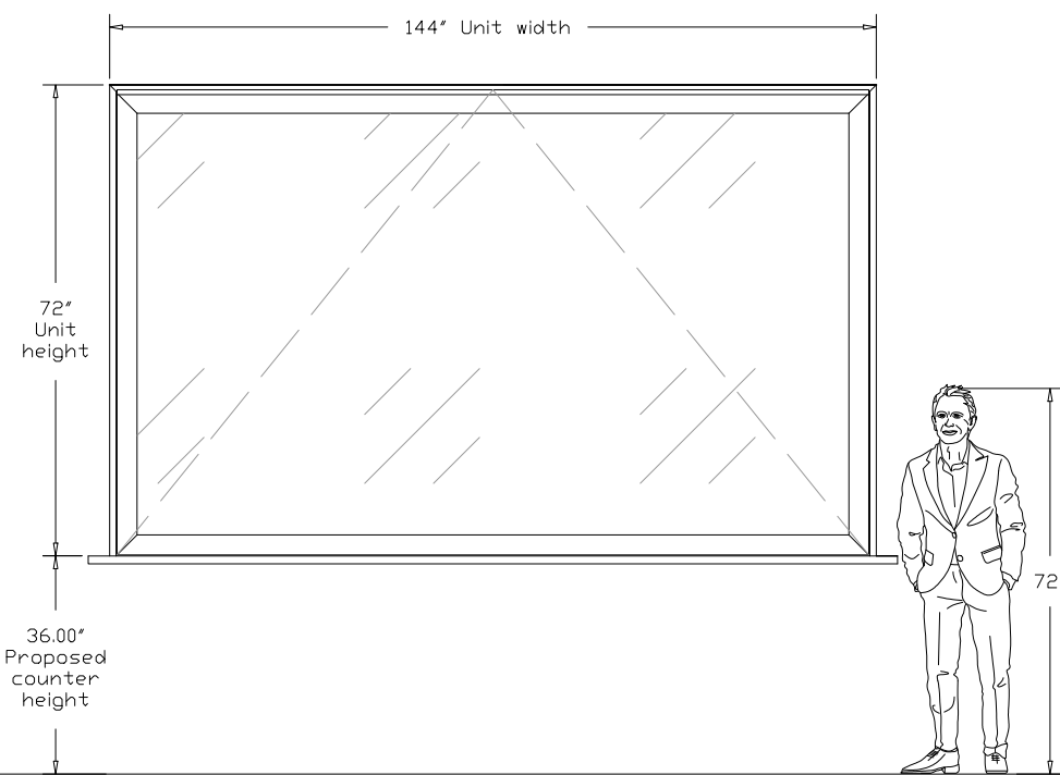
Exterior Elevation
