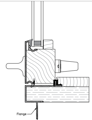
Full Bound Jamb/Sill
