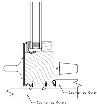
Step Sill Counter by Others
