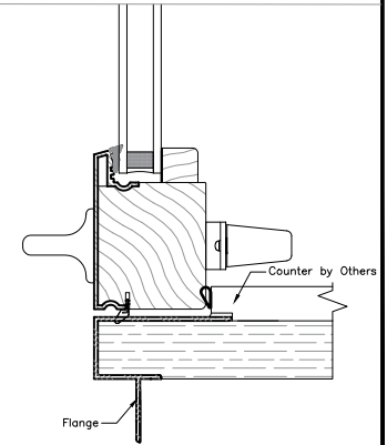
Hybrid Full Bound Jamb/Sill
