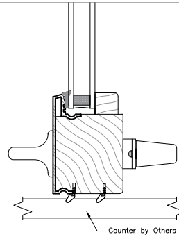
Flush Sill Counter by Others
