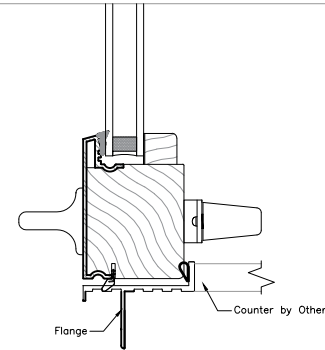
Minimal Aluminum Sill
