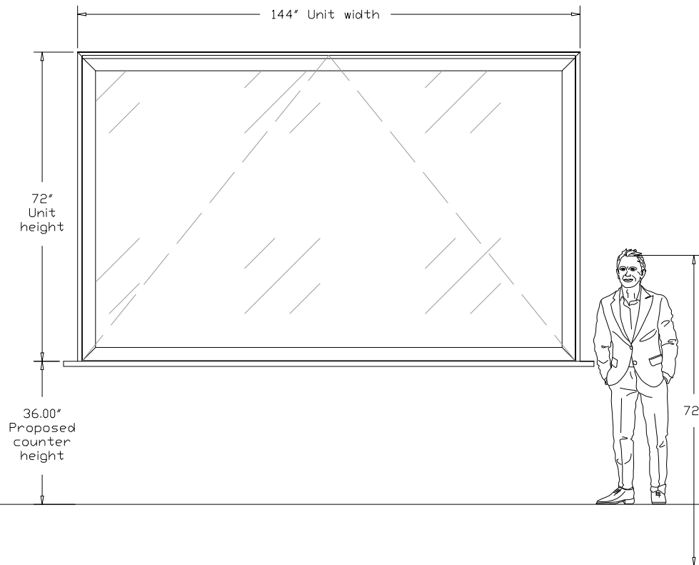
Exterior Elevation
